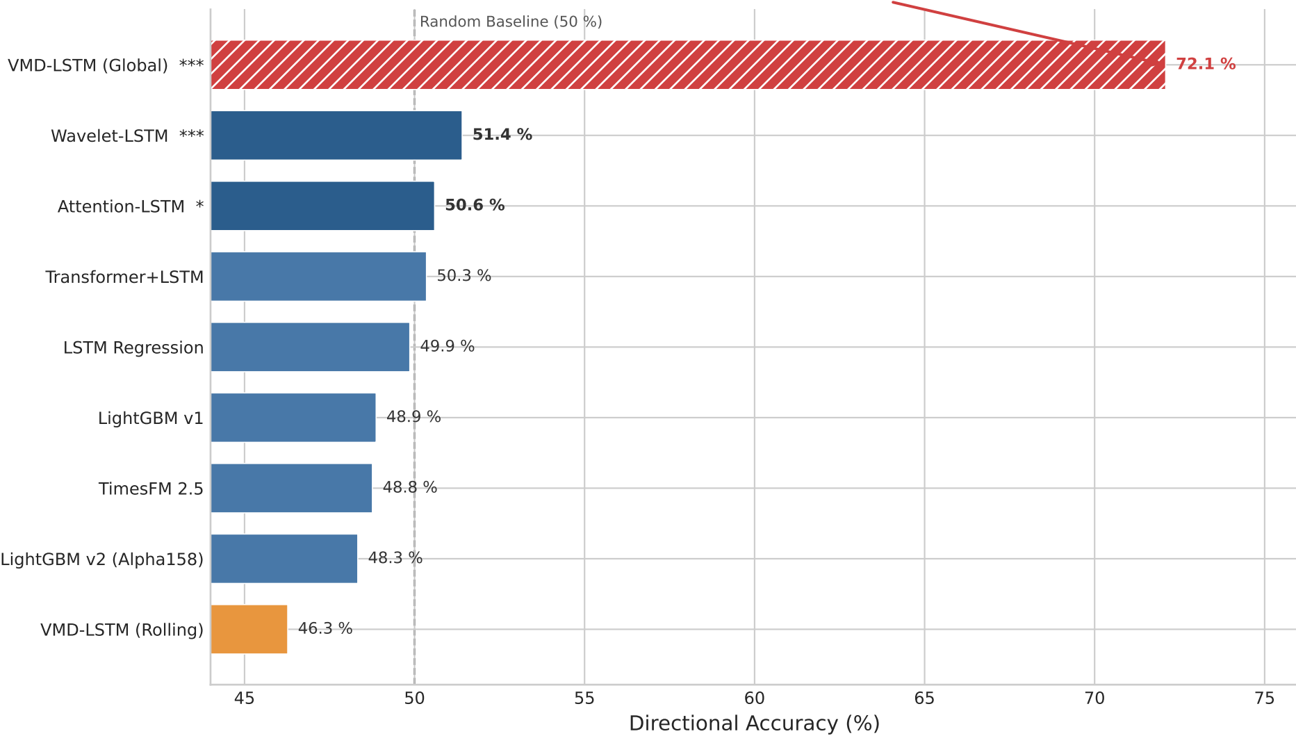
Figure 4.1a: Directional Accuracy of Direct Prediction Models
