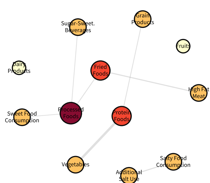
Female Middle MetS(-) (N=5629, Edges=7, Density=10.6%)
