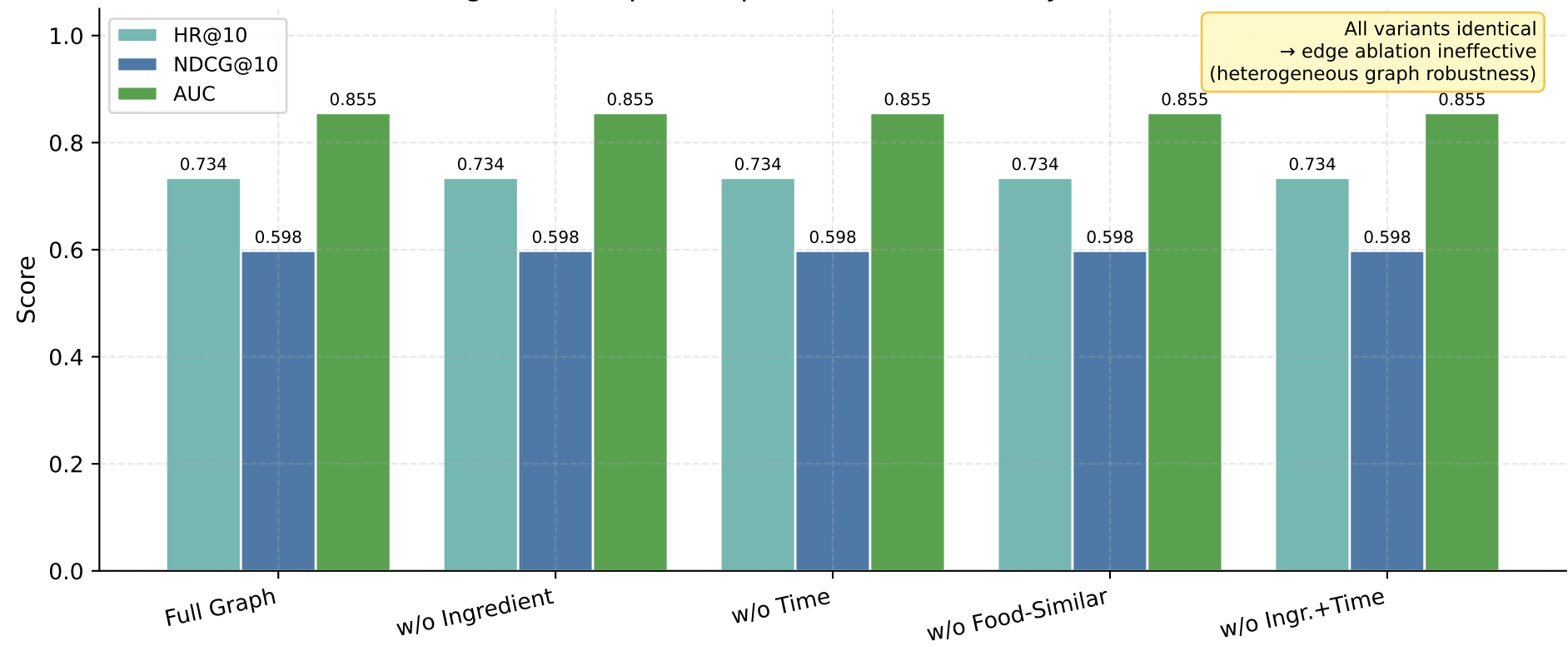
Figure 5. Graph Component Ablation Study (HFRS-DA)
