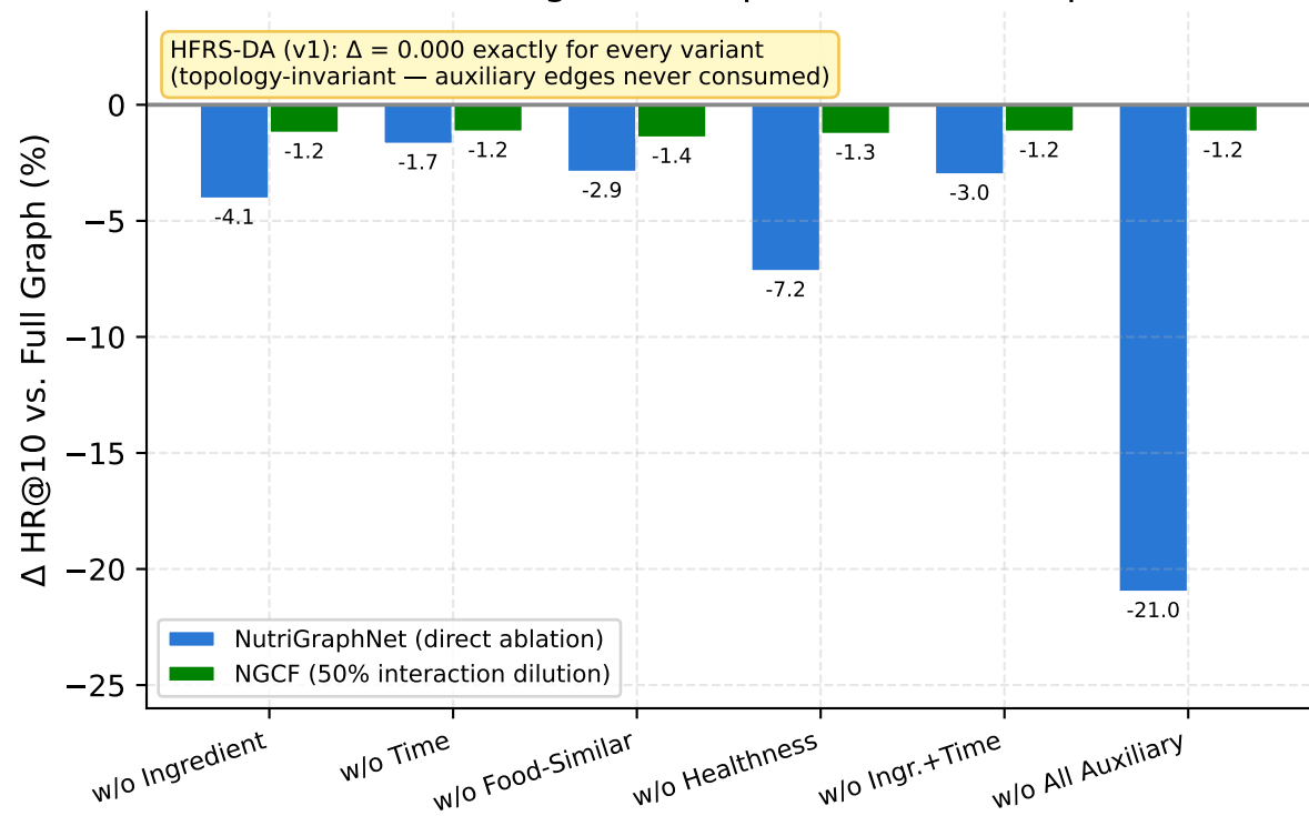
(b) Relative Degradation per Ablated Component
