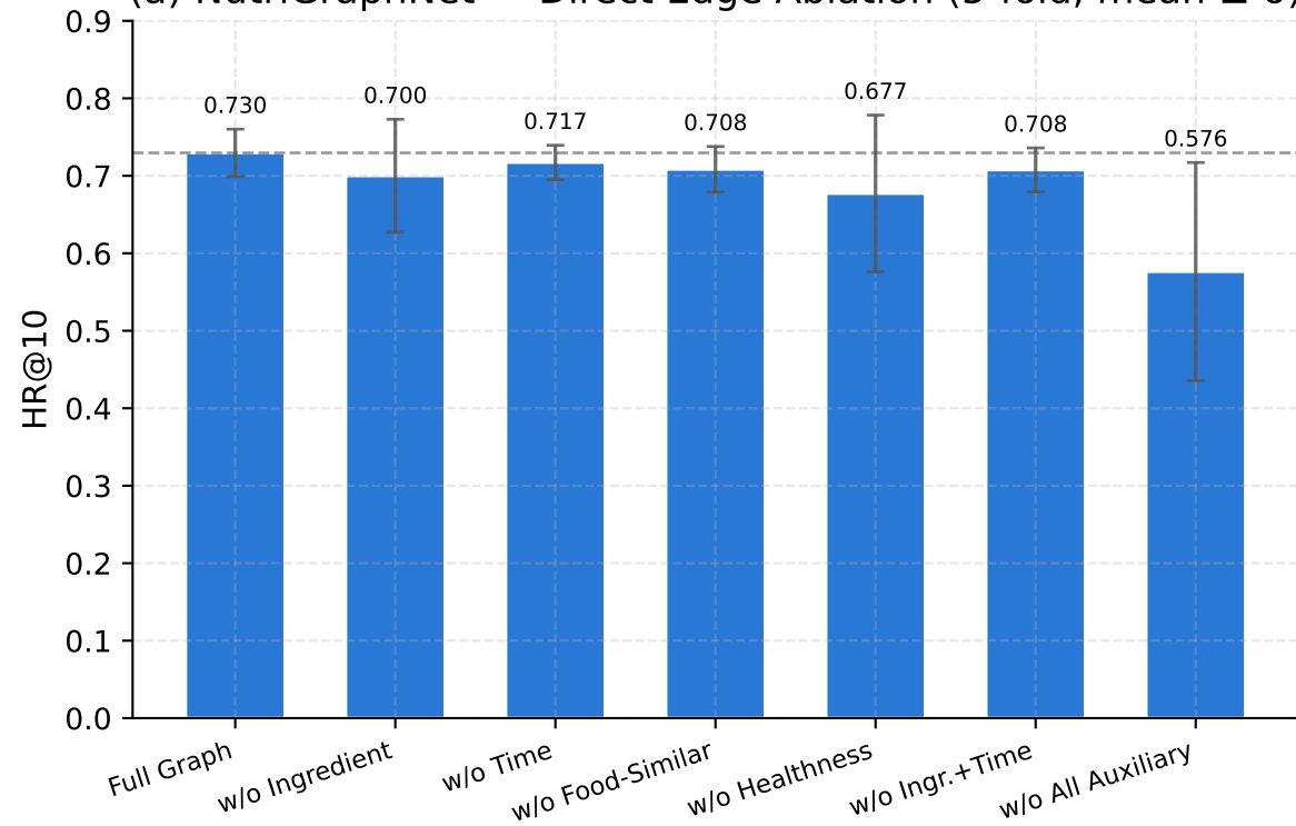
(a) NutriGraphNet — Direct Edge Ablation (5-fold, mean \pm \sigma )
