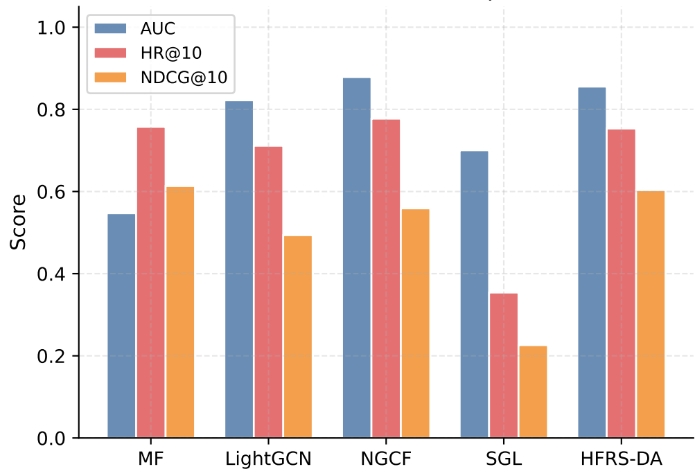
(b) Full-Data Metric Profile per Model
