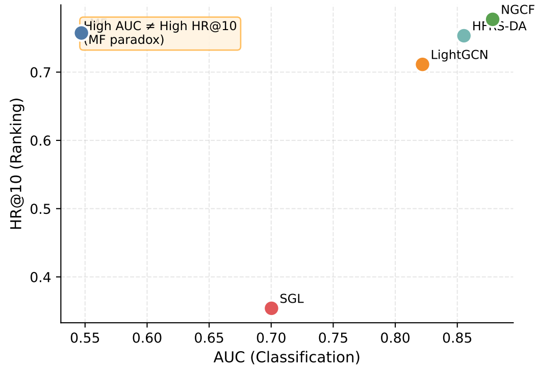
(a) AUC vs. HR@10 — Score Paradox
