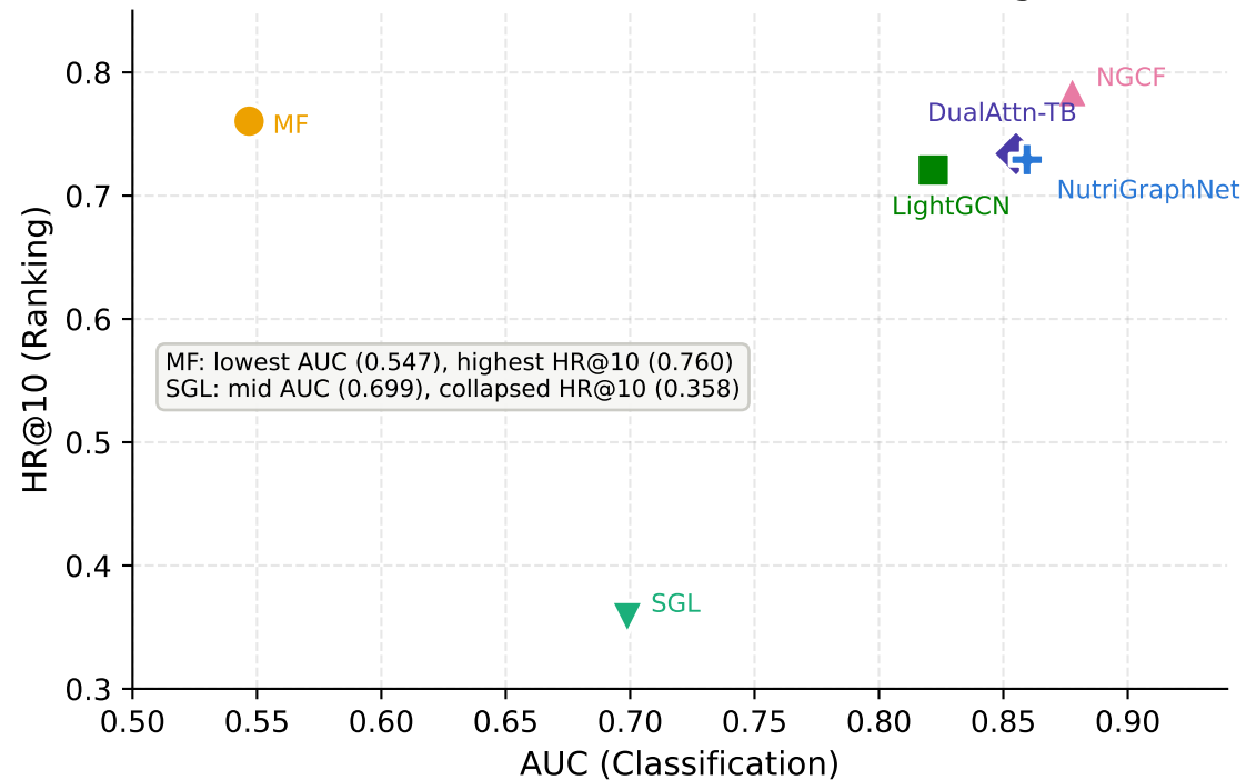
(a) AUC vs. HR@10 — the two do not agree
