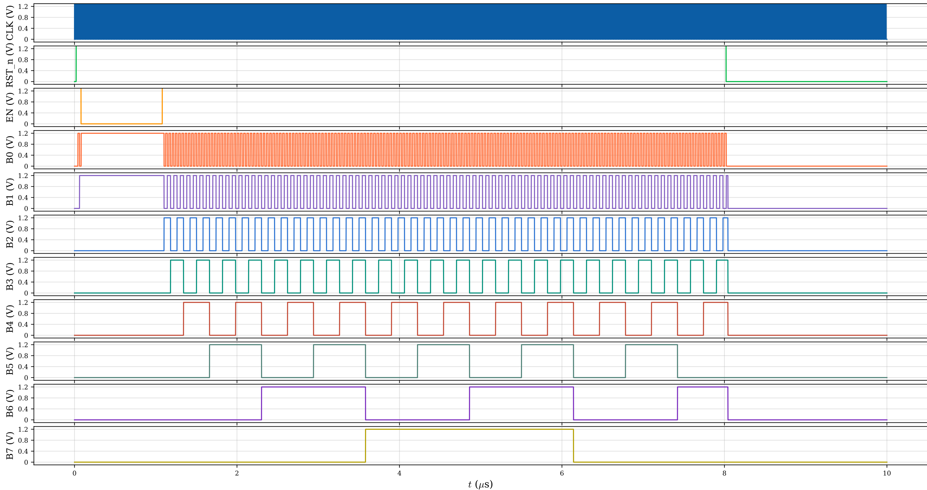
Counter - Gate-Level Transient Simulation
