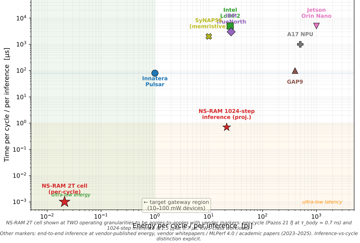
Figure 1: NS-RAM 2T cell, two-granularity positioning against published edge-AI baselines. The lower red star is the per-cycle measurement (Pazos: 21 fJ at \tau_{\text{body}} \approx 0.7 ns), the upper red star is a device-only projection of 1024 \times 21 fJ at 1024 \times 0.7 ns = 0.7 \mu s for a KWS-class inference. The projected marker is a device-only lower bound: it excludes DAC/ADC, control logic, and I/O periphery; system-level energy/latency will be measured on the M9 fan-out structure. Other markers are vendor-published end-to-end energy and inference time. Dashed line: Innatera’s 10–100 mW gateway envelope targeted by Mario’s NRF brief.
