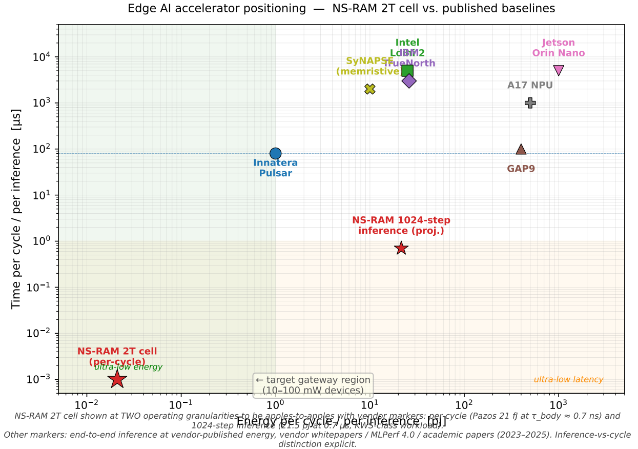
Figure 1: NS-RAM 2T cell, two-granularity positioning against published edge-AI baselines. The lower red star is the per-cycle measurement (Pazos: 21 fJ at the \approx 0.7 ns avalanche-pulse front), the upper red star is a device-only projection of 1024 \times 21 fJ at 1024 \times 0.7\text{ ns} = 0.7\text{ }\mu\text{s} for a KWS-class (keyword-spotting) inference. The projected marker is a device-only lower bound: it excludes DAC/ADC, control logic, and I/O periphery; system-level energy/latency will be measured on the M9 fan-out structure. Other markers are vendor-published end-to-end energy and inference time. Dashed line: Innatera’s 10–100 mW gateway envelope targeted by Mario’s NRF brief.
