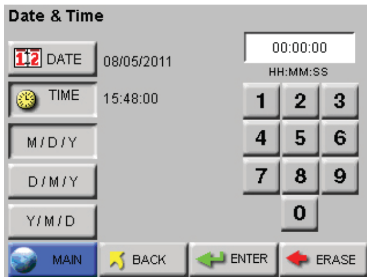
Figure 6-40 Configuring TIME
