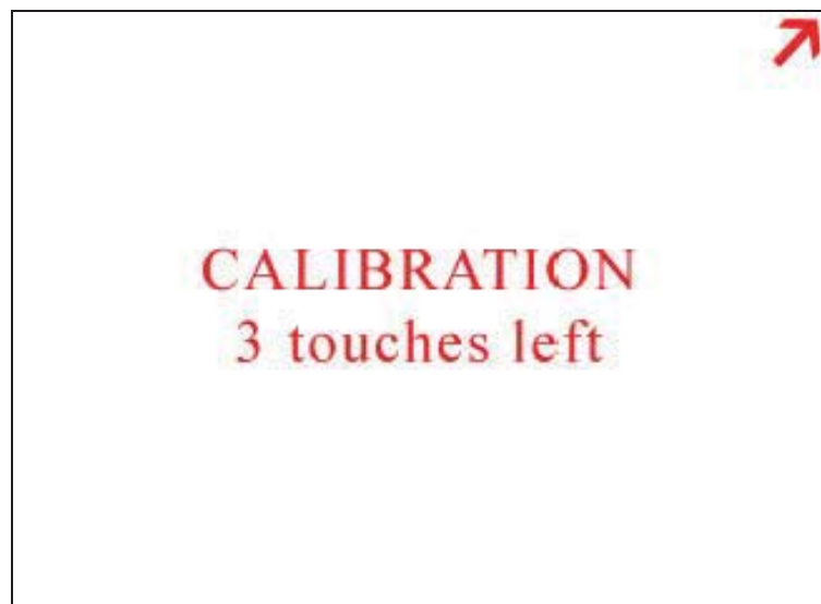
Figure 6-43 Alignment Screen 2
