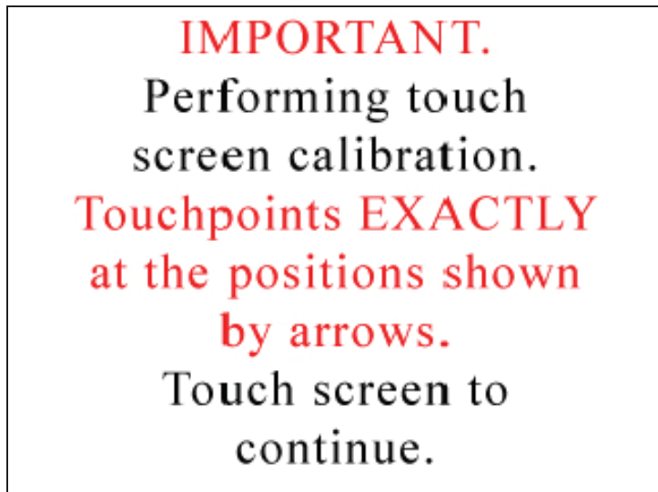
Figure 6-42 Alignment Screen 1
