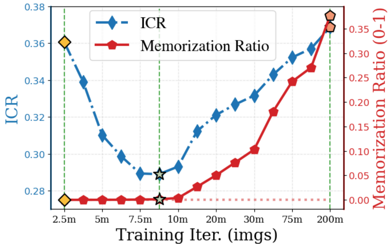
CIFAR10 (training set size: 4,096 images)
