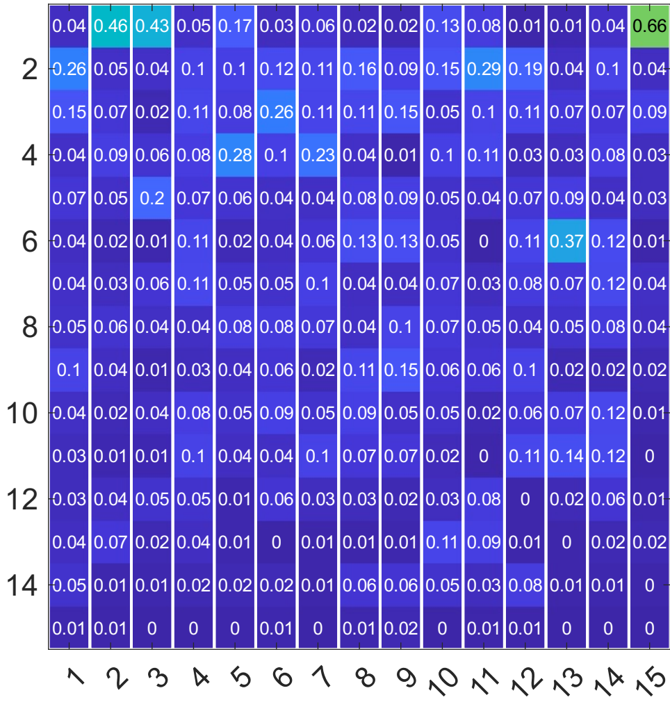
Channel Feat.
