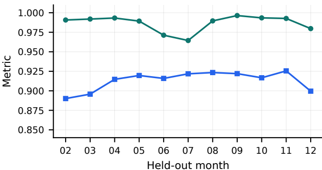
(a) Rolling PE-KB validation
