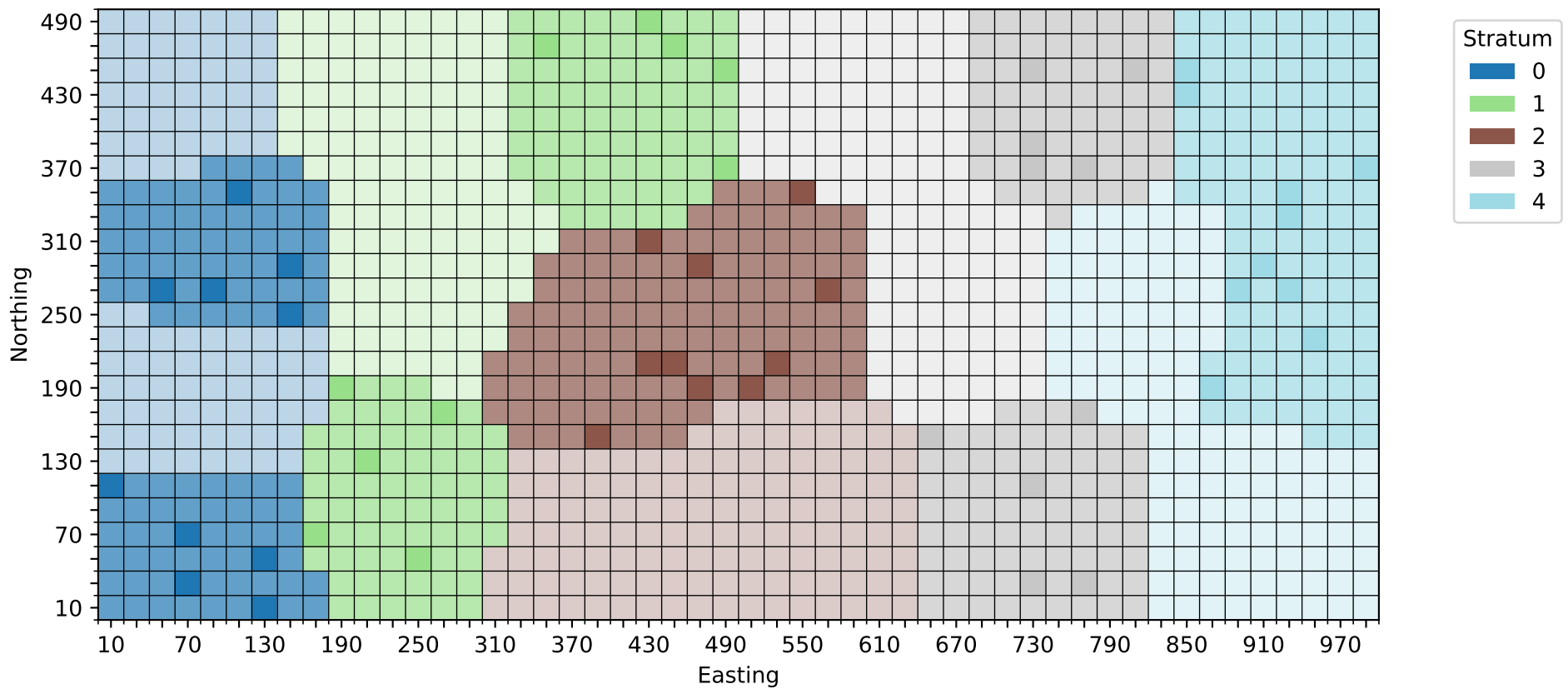
Soil Data Clustering (Strata)
