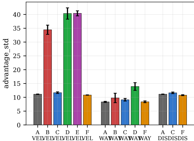
advantage_std (GAE) plateau
