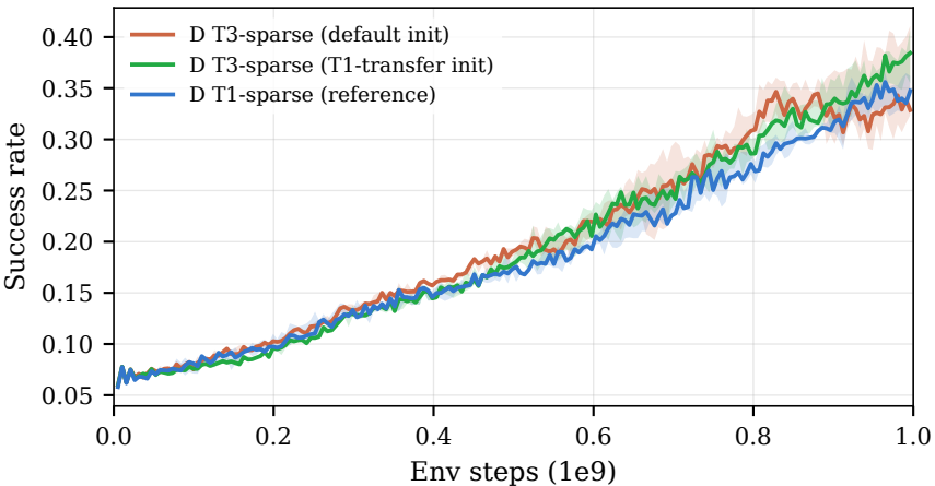
E1 cross-task PSC weight transfer (T3-sparse)
