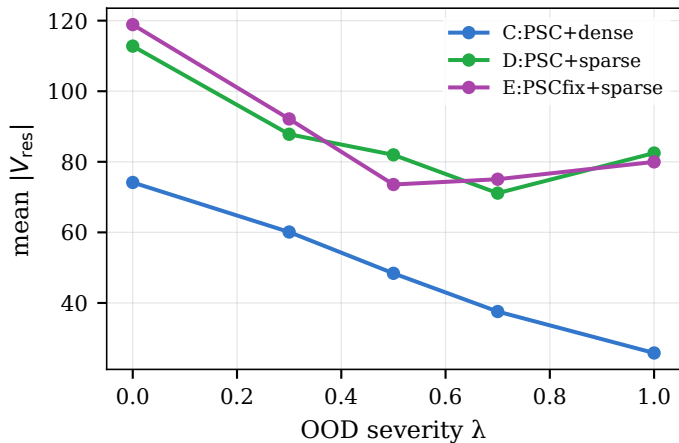
|V_{\text{res}}| vs \lambda
