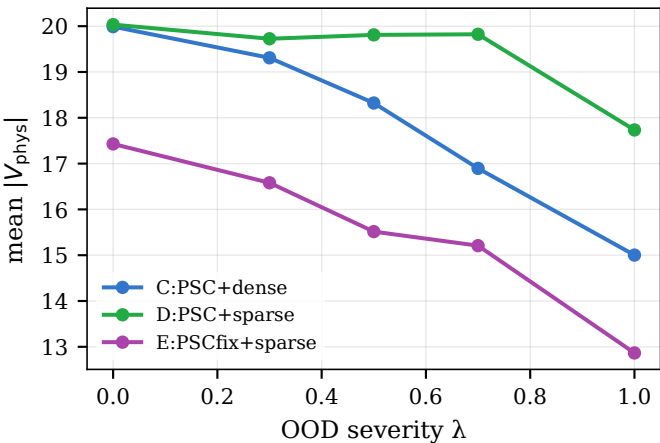
|V_{\text{phys}}| vs \lambda
