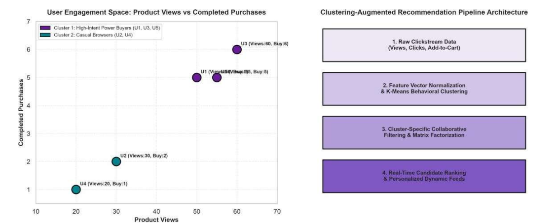
Figure 2.4: (Left) User engagement feature space mapping Views against Completed Purchases; (Right) 4-Stage Clustering-Augmented Recommendation Engine Architecture.
