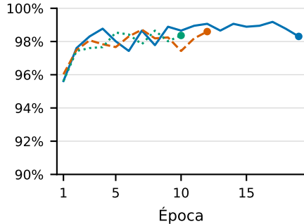
ResNet18
