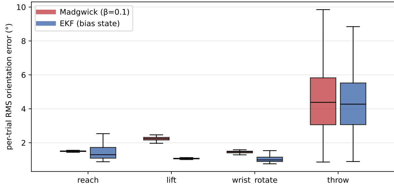
Orientation error by motion class (1000 trials, 3 sensors each)
