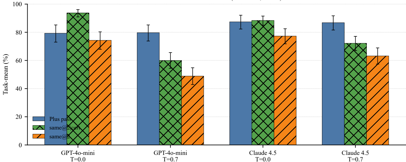
SameEval on HumanEval+ (164 tasks, N=20)
