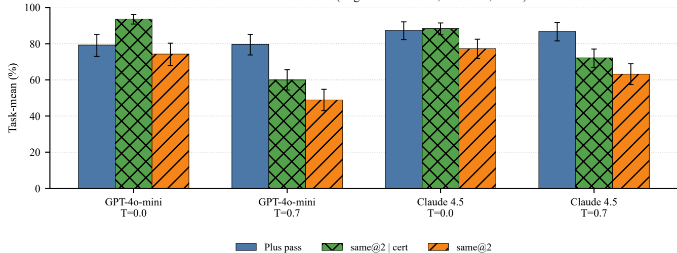
SameEval on HumanEval+ (original two models, 164 tasks, N=20)
