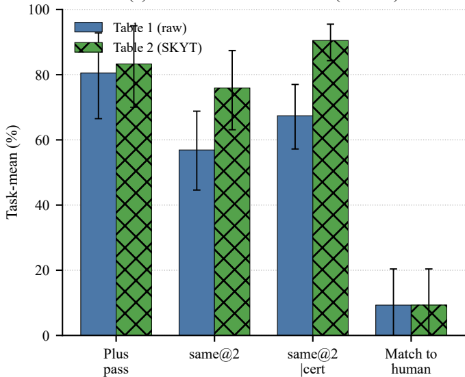
(b) SameEval on HumanEval+ (30 tasks)
