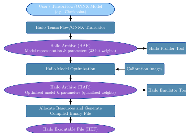
Figure 2.4: Build Process [17]
