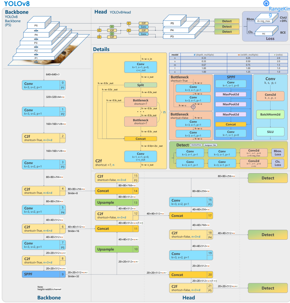
Figure 2.1: Overall YOLOv8 architecture and model scaling variables [39]
