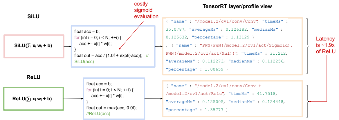
Figure 5.5: Comparison of TensorRT per-layer profiling for convolution followed by SiLU and ReLU. In the ReLU case, TensorRT reports a fused Conv + Relu region, whereas in the SiLU case the activation appears as additional pointwise Sigmoid and Mul operations. For the profiled example, the convolution time remains similar, but the extra SiLU activation work increases the total layer cost to approximately 1.9× that of the fused ReLU case.
