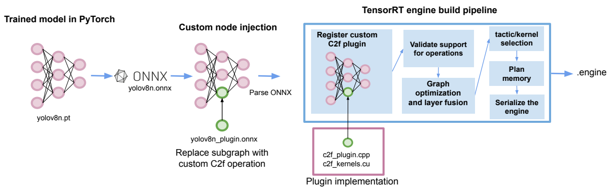
Figure 5.4: TensorRT engine build workflow with custom plugin injection. A trained YOLOv8 model is exported from PyTorch to ONNX, a selected C2f subgraph is replaced by a custom plugin node, and TensorRT builds a target-specific engine by parsing the modified graph, validating supported operators and registered plugins, applying graph optimizations, selecting tactics, planning memory, and serializing the final engine
