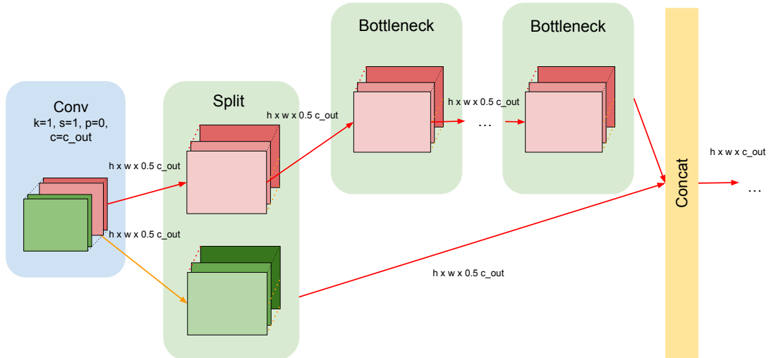
Figure 5.3: Data flow and channel dependencies within the C2f block.
