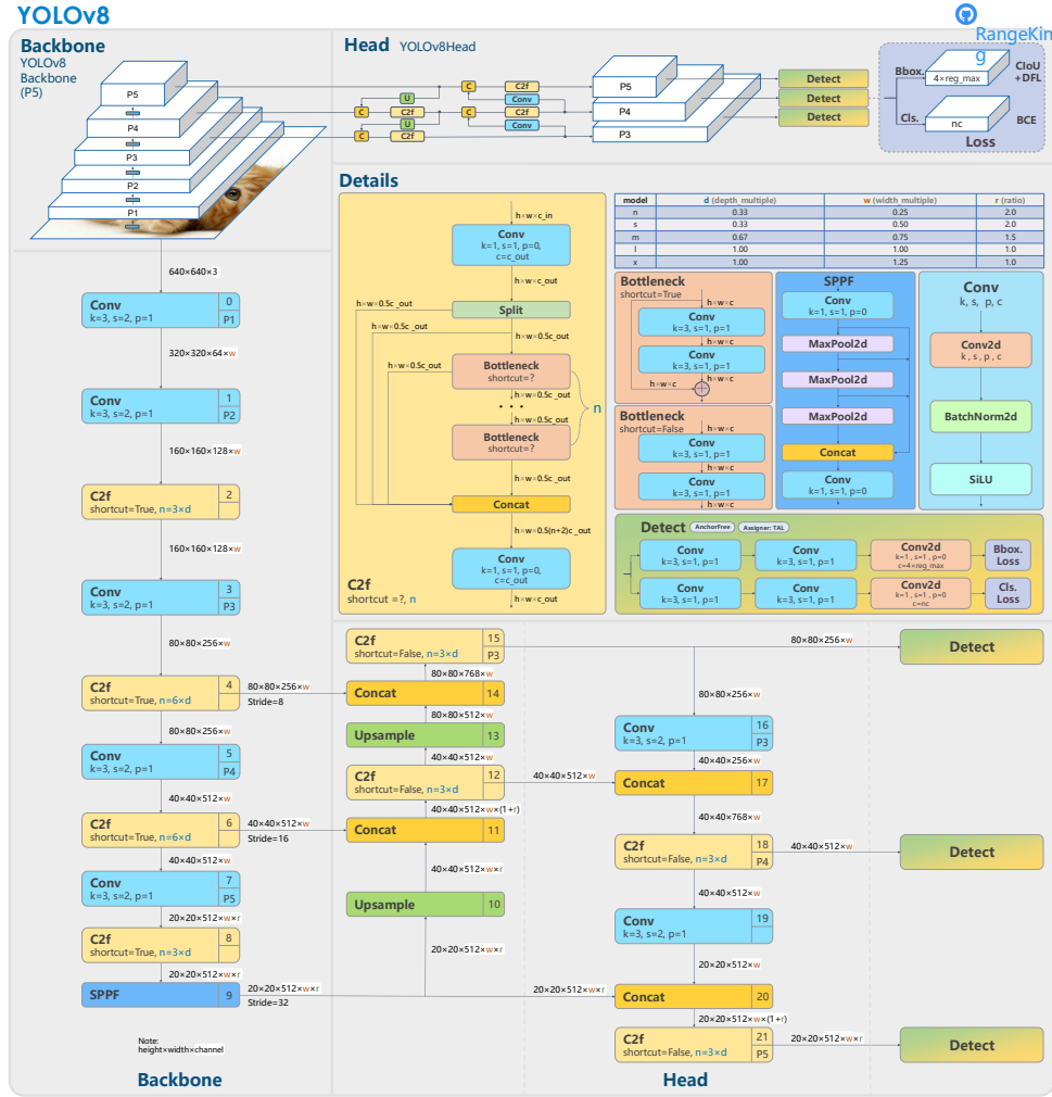
Figure 2.1: Overall YOLOv8 architecture and model scaling variables [2]
