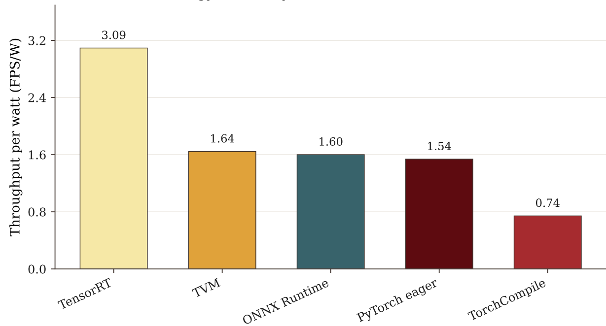
Energy efficiency of YOLOv8n FP32 inference
