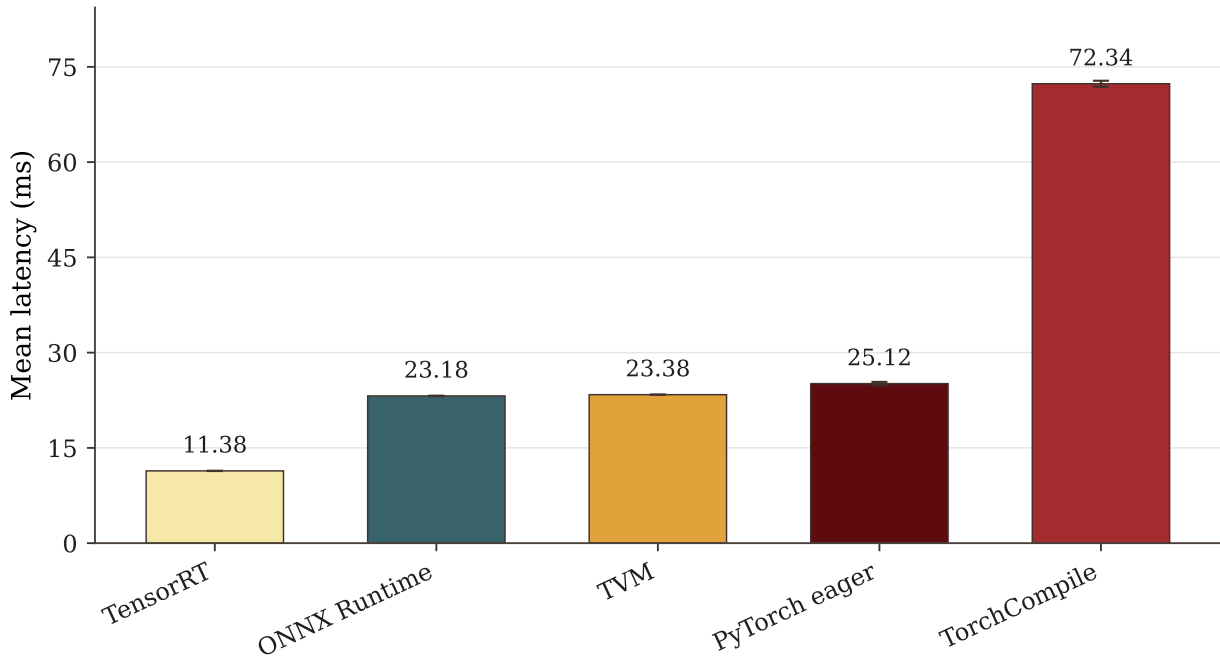
YOLOv8n FP32 inference latency on Jetson Orin Nano GPU
