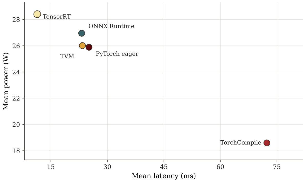
Latency-power trade-off on Jetson Orin Nano GPU
