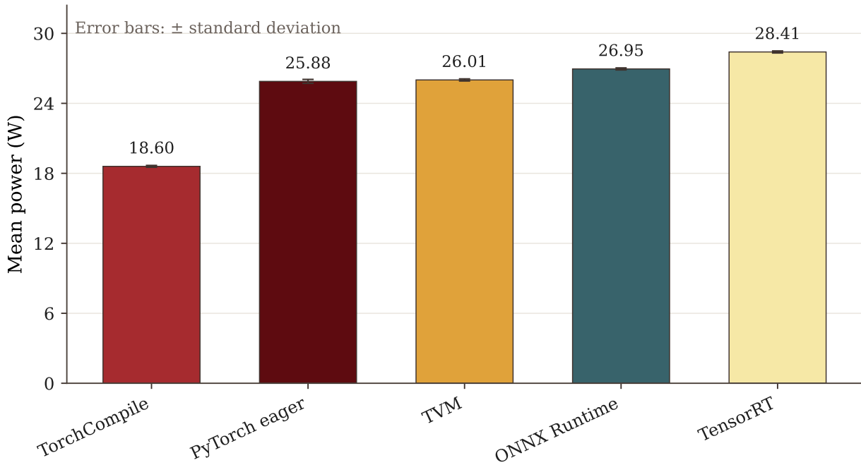
Power consumption during YOLOv8n FP32 inference
