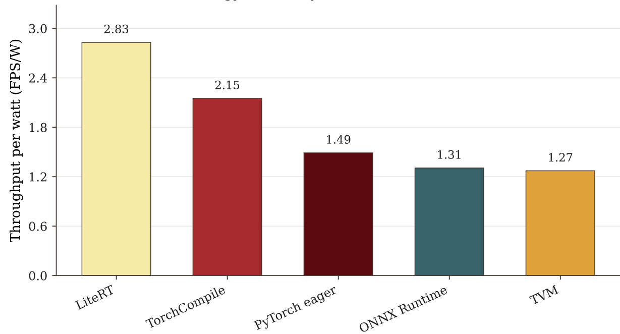
Energy efficiency of YOLOv8n inference
