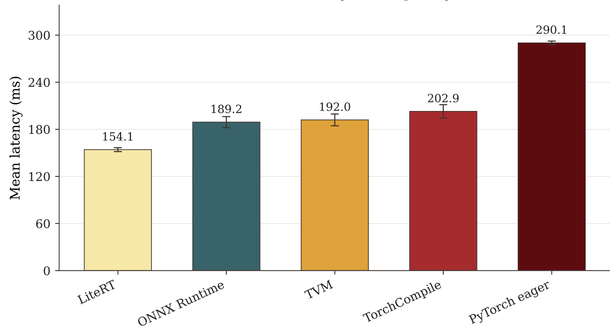
YOLOv8n inference latency on Raspberry Pi 5 CPU
