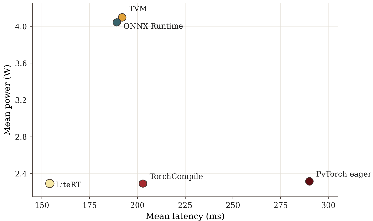
Latency-power trade-off on Raspberry Pi 5 CPU
