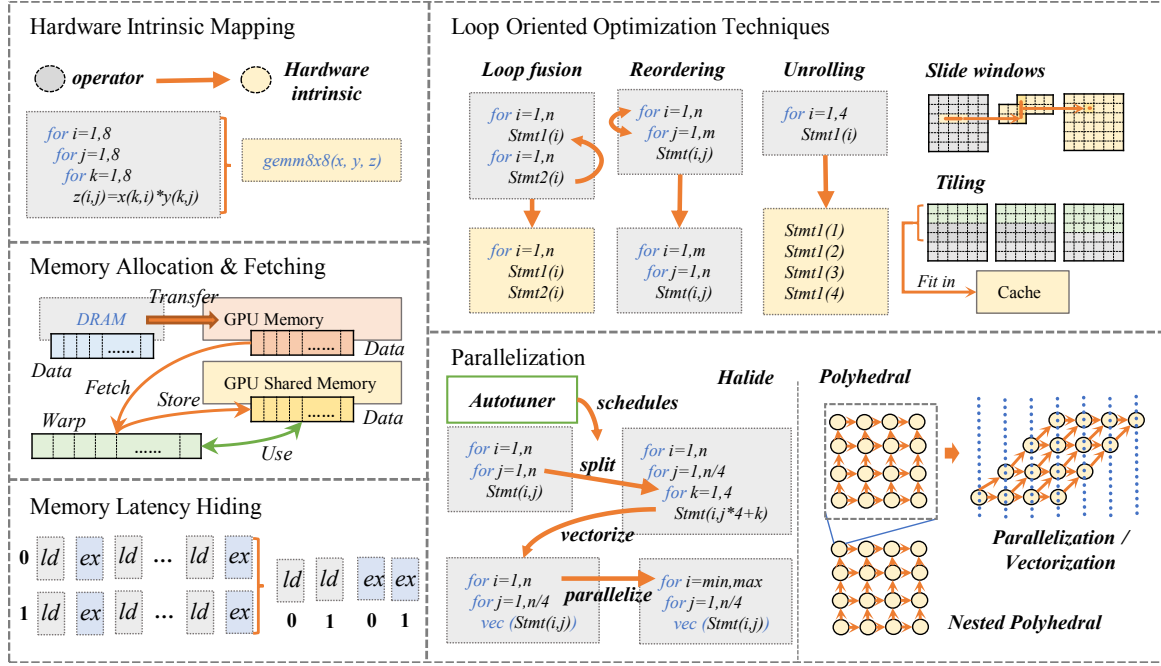
Figure 2.3: Overview of hardware-specific optimizations applied in deep-learning compilers. Reproduced from Li et al. [24].
