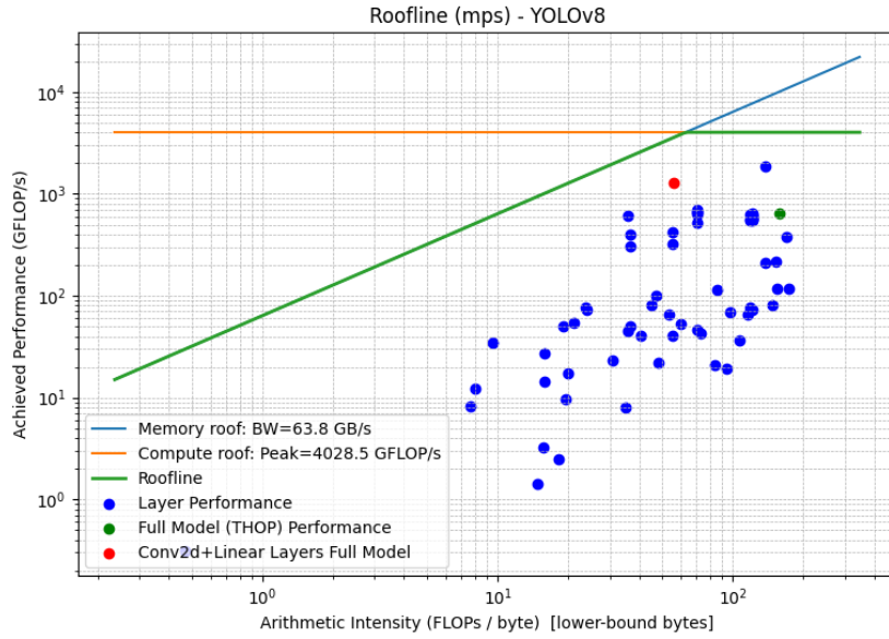
Figure 5.3: Roofline model of YOLOv8n on Macbook Pro M3 (MPS, FP32).
