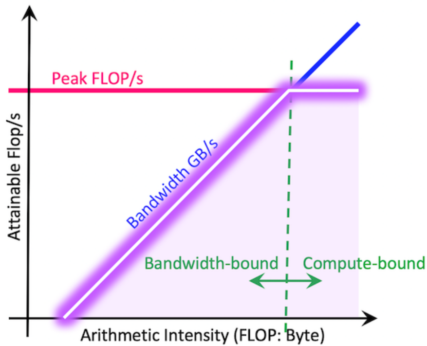
Figure 2.2: A Roofline model illustrating performance limits based on compute capability (horizontal line) and memory bandwidth (sloped line) versus the arithmetic intensity of operations (dots). Operations below the "roof" are limited by either memory bandwidth or compute peak.
