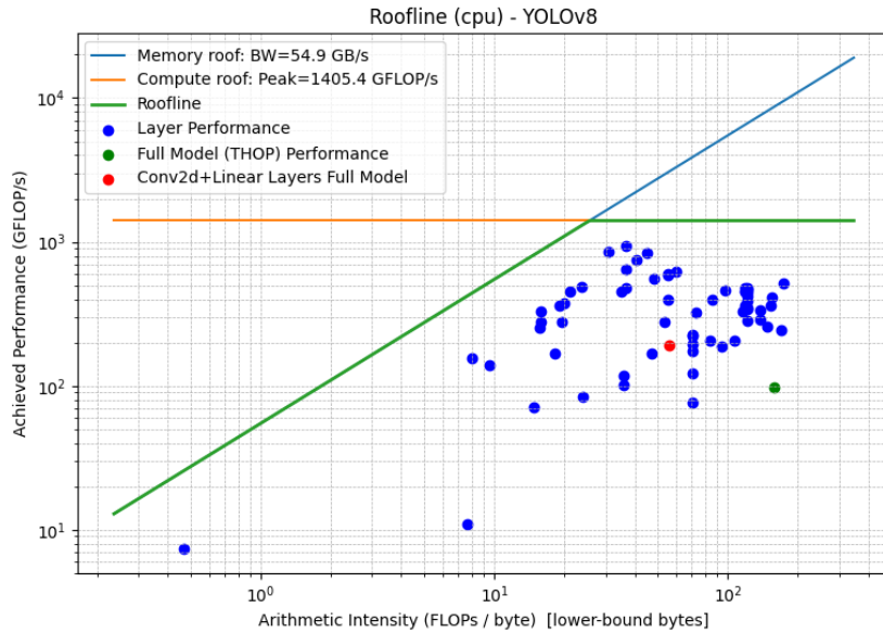
Figure 5.2: Roofline model of YOLOv8n on Macbook Pro M3 (CPU, FP32).
