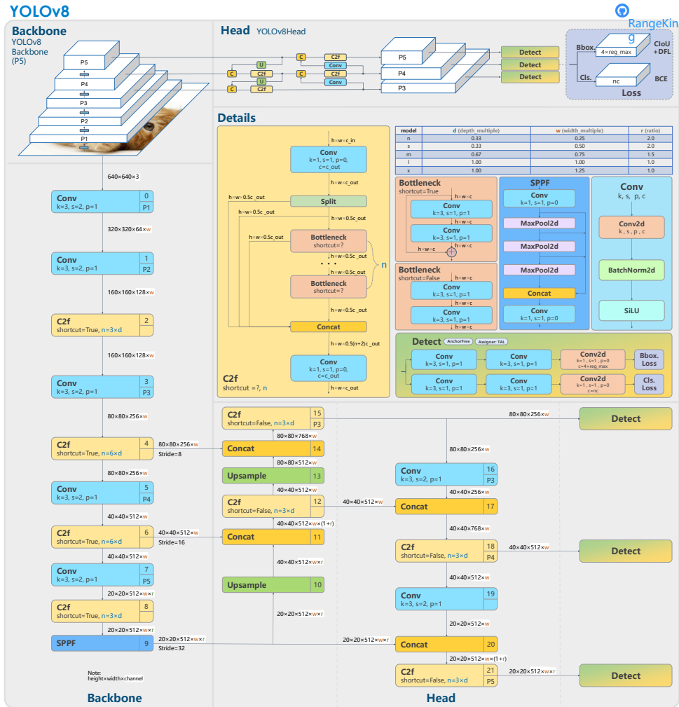
Figure 2.1: Overall YOLOv8 architecture and model scaling variables [35]
