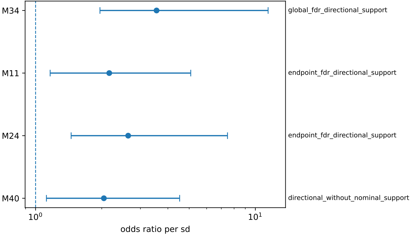
GSE21257: frozen program association with metastasis within five years
