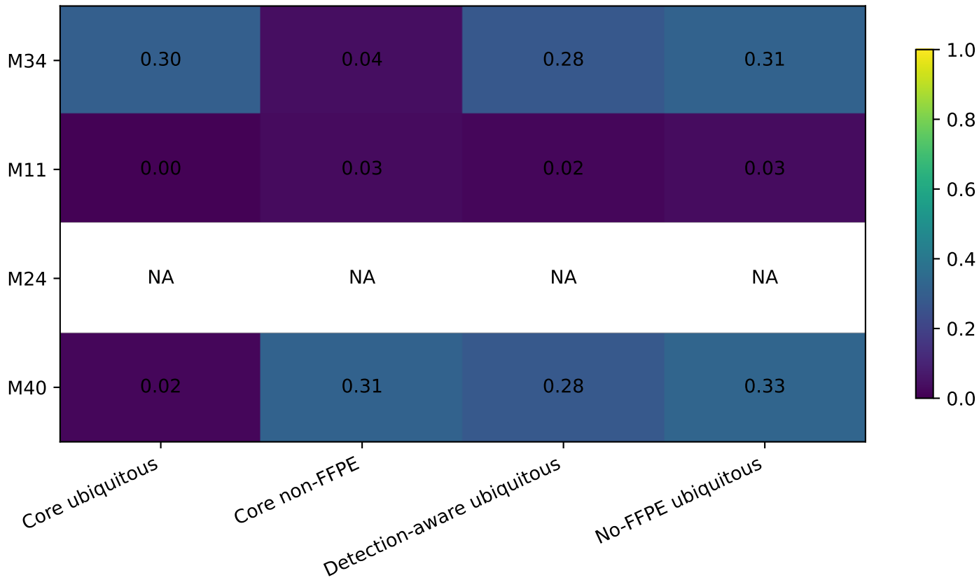
Variable-only MOFA: frozen-module latent-subspace capture
