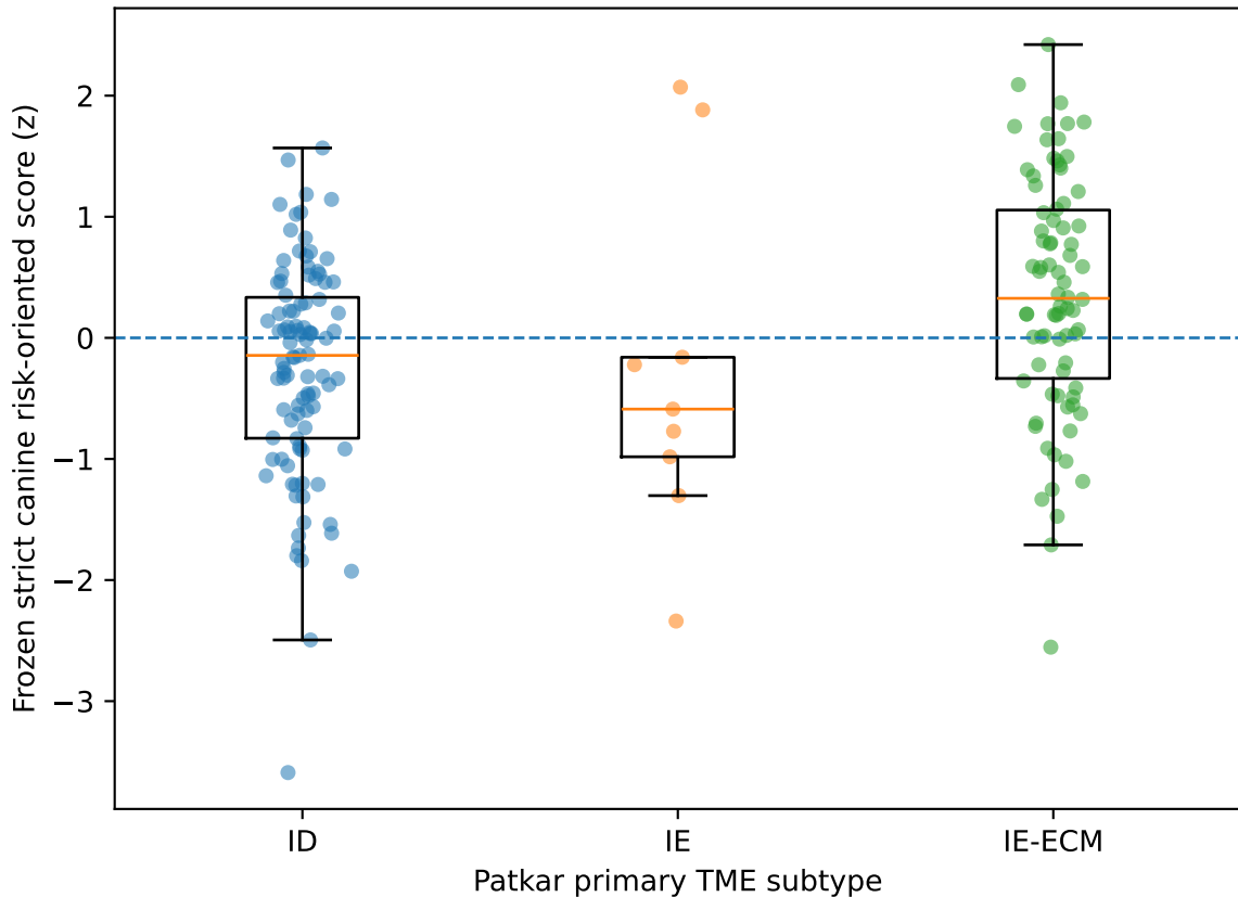
M11: frozen program score across Patkar TME subtypes
