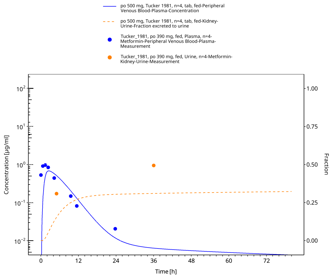
Figure 3-23: Metformin - po (tab) 500 mg_Tucker 1981
