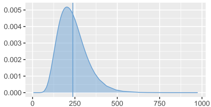
Precision of beta
