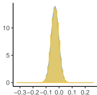
Epsilon[96], Inlabru ar
