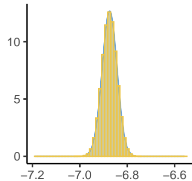
Predictor[162]
