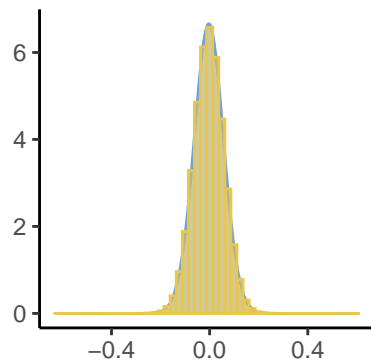
Epsilon[1]
