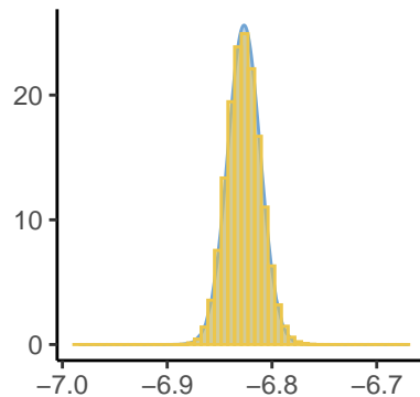
Predictor[32]
