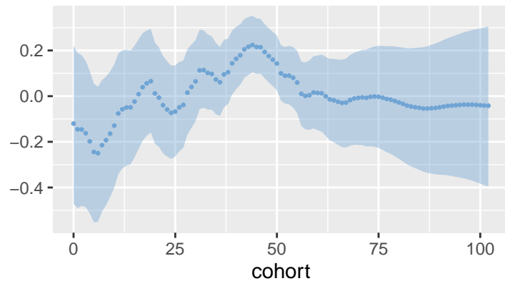
Gamma
