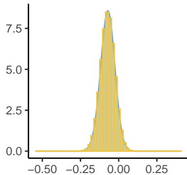
Epsilon[192], Inlabru a
