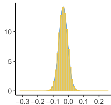
Epsilon[64], Inlabru and stan
