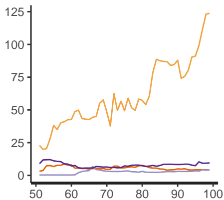
intercept
