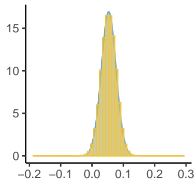
Epsilon[32]
