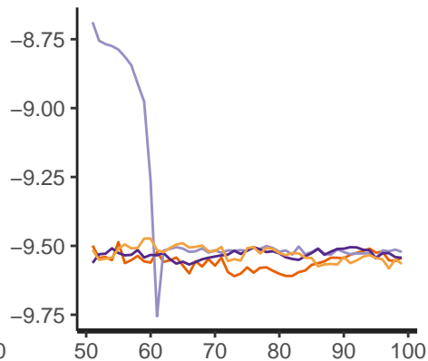
intercept
