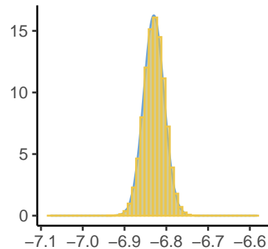
Predictor[162]
