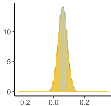
Epsilon[32], Inlabru and
