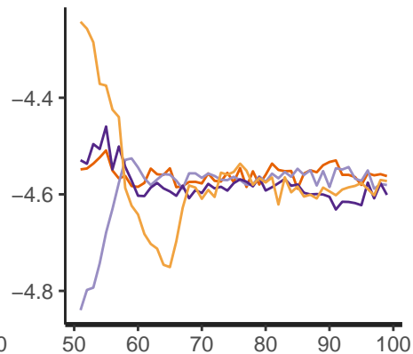
intercept
