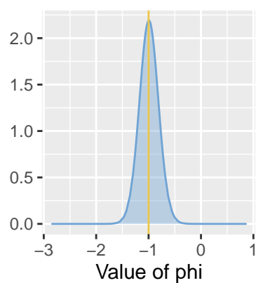
Drift term – inlabru
