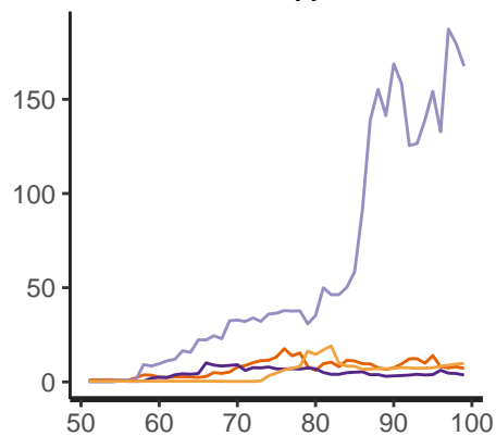
intercept
