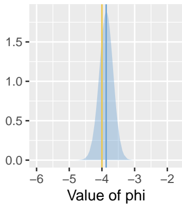
Phi*t + kappa
