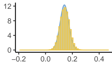
Beta[7]
