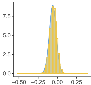
Epsilon[256]
