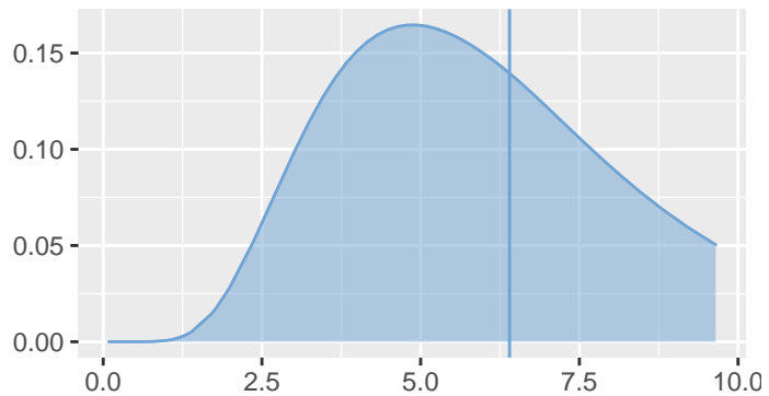
Precision of alpha
