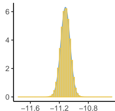
Predictor[64], Inlabru and stan
