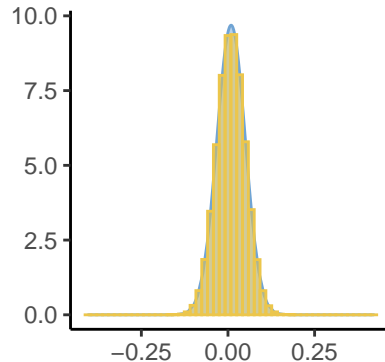
Epsilon[128], Inlabru a
