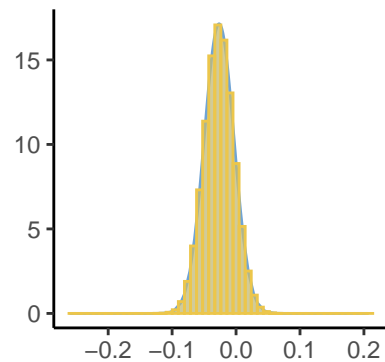
Epsilon[64]
