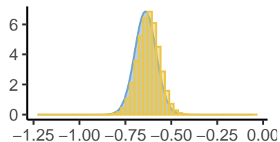
Kappa[3]
