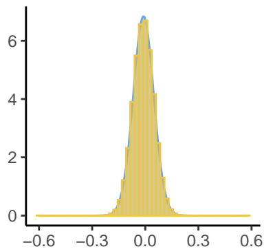
Epsilon[64], Inlabru and
