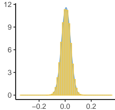
Epsilon[128]
