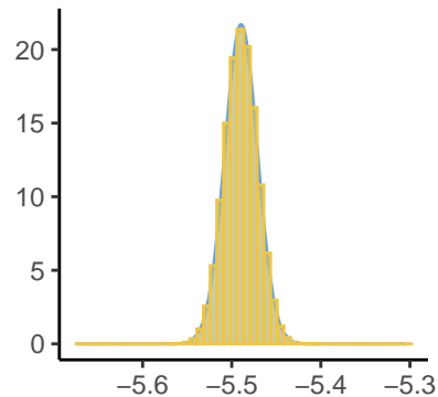
Predictor[324]
