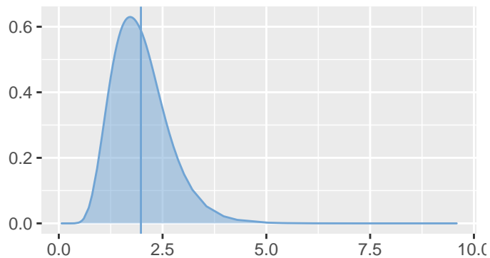
Precision of alpha
