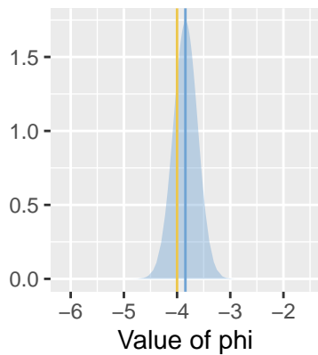
Phi*t + kappa
