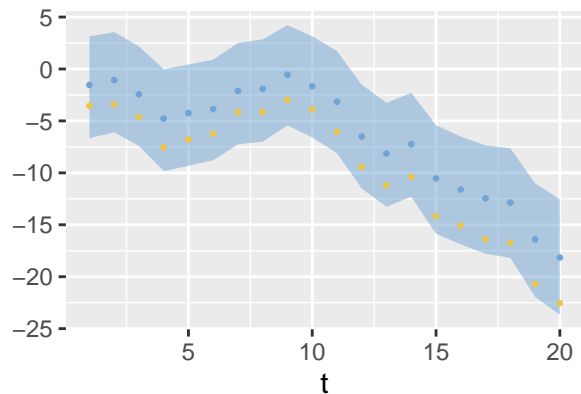
Phi*t + kappa
