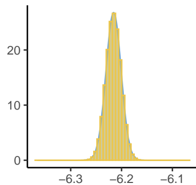
Predictor[64]
