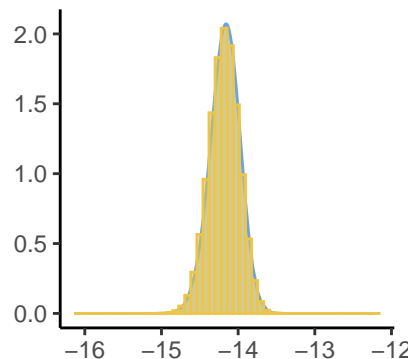
Predictor[32], Inlabru a
