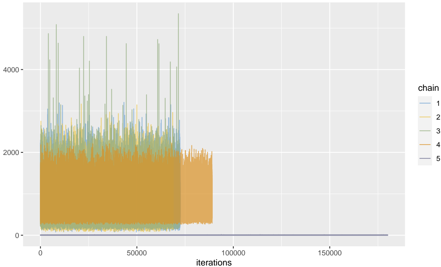
Trace plot Precision of Beta – lung cancer, male
