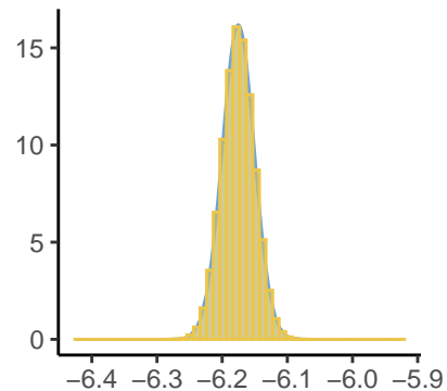
Predictor[64]
