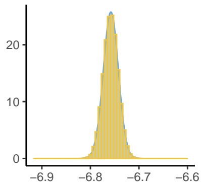
Predictor[32]
