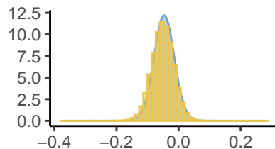
Beta[3]
