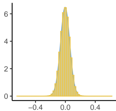
Epsilon[1], Inlabru and
