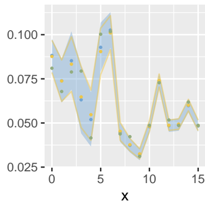
Beta
