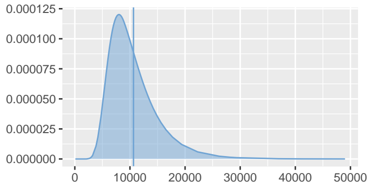
Precision of epsilon
