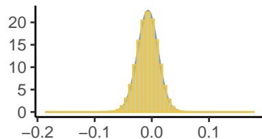
Kappa[3], Inlabru and stan
