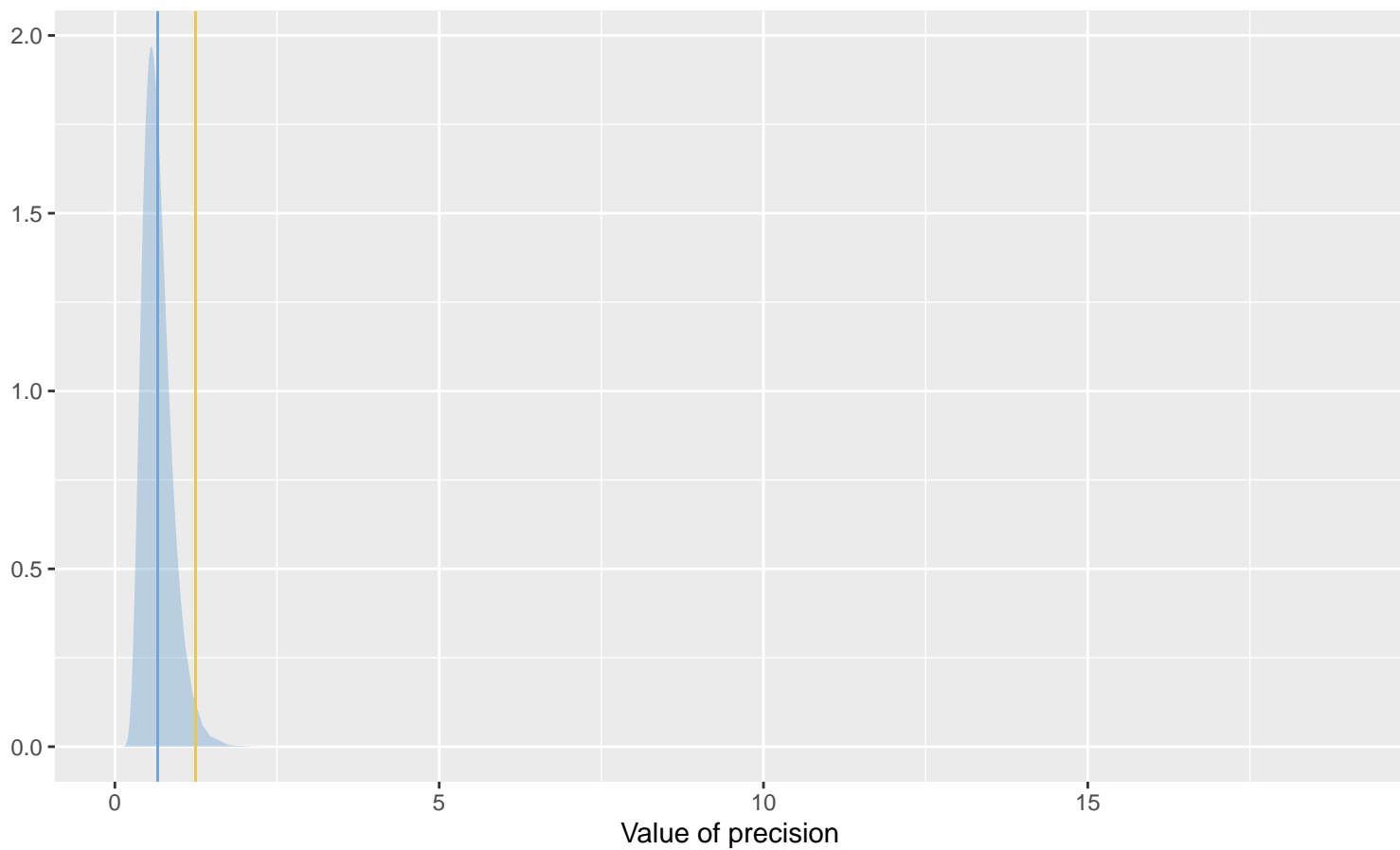
Precision for kappa – comparison
