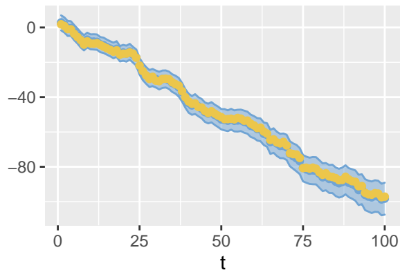
Phi*t + kappa
