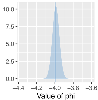
Phi*t + kappa
