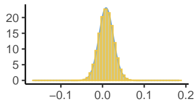
Kappa[13], Inlabru and stan
