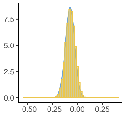
Epsilon[128]
