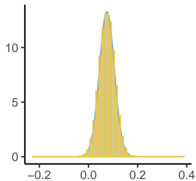
Epsilon[1], Inlabru and
