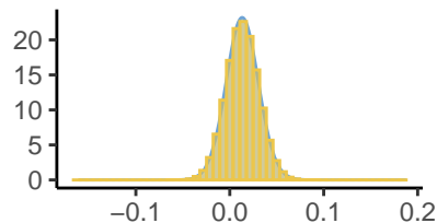
Kappa[7], Inlabru and stan
