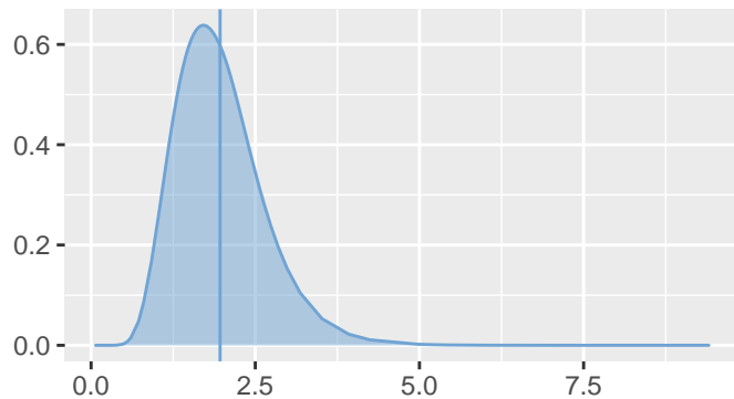
Precision of alpha
