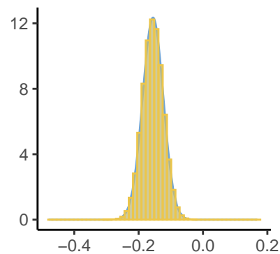
Epsilon[162]
