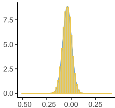
Epsilon[256], Inlabru a
