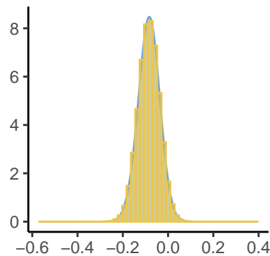
Epsilon[128], Inlabru and stan
