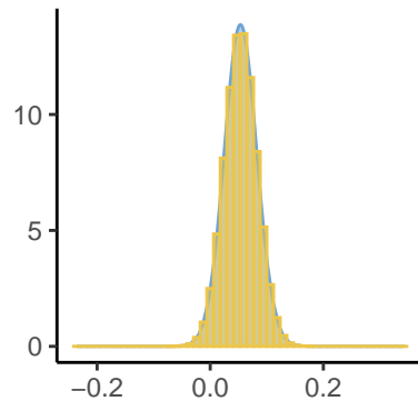
Epsilon[324], Inlabru ar
