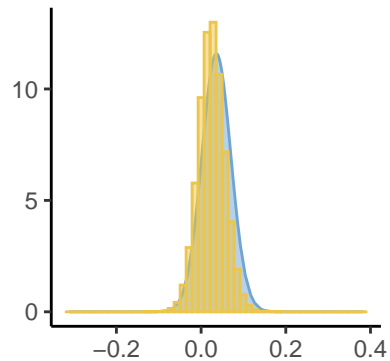
Epsilon[324]
