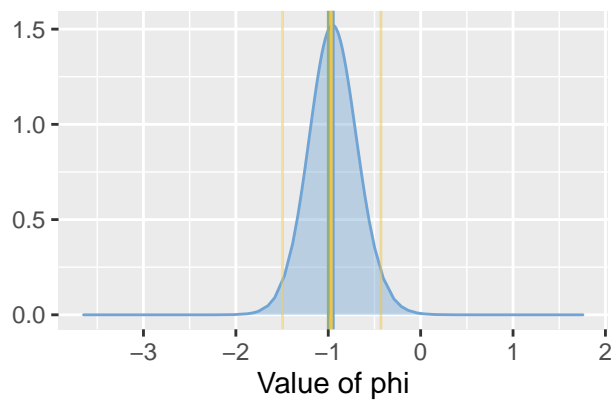
Phi
