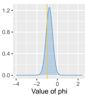
Drift term – inlabru
