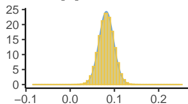
Beta[2]
