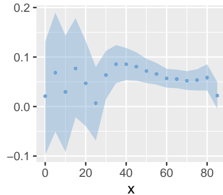
Beta
