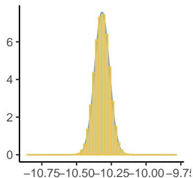
Predictor[96], Inlabru a
