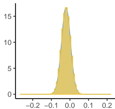
Epsilon[96]
