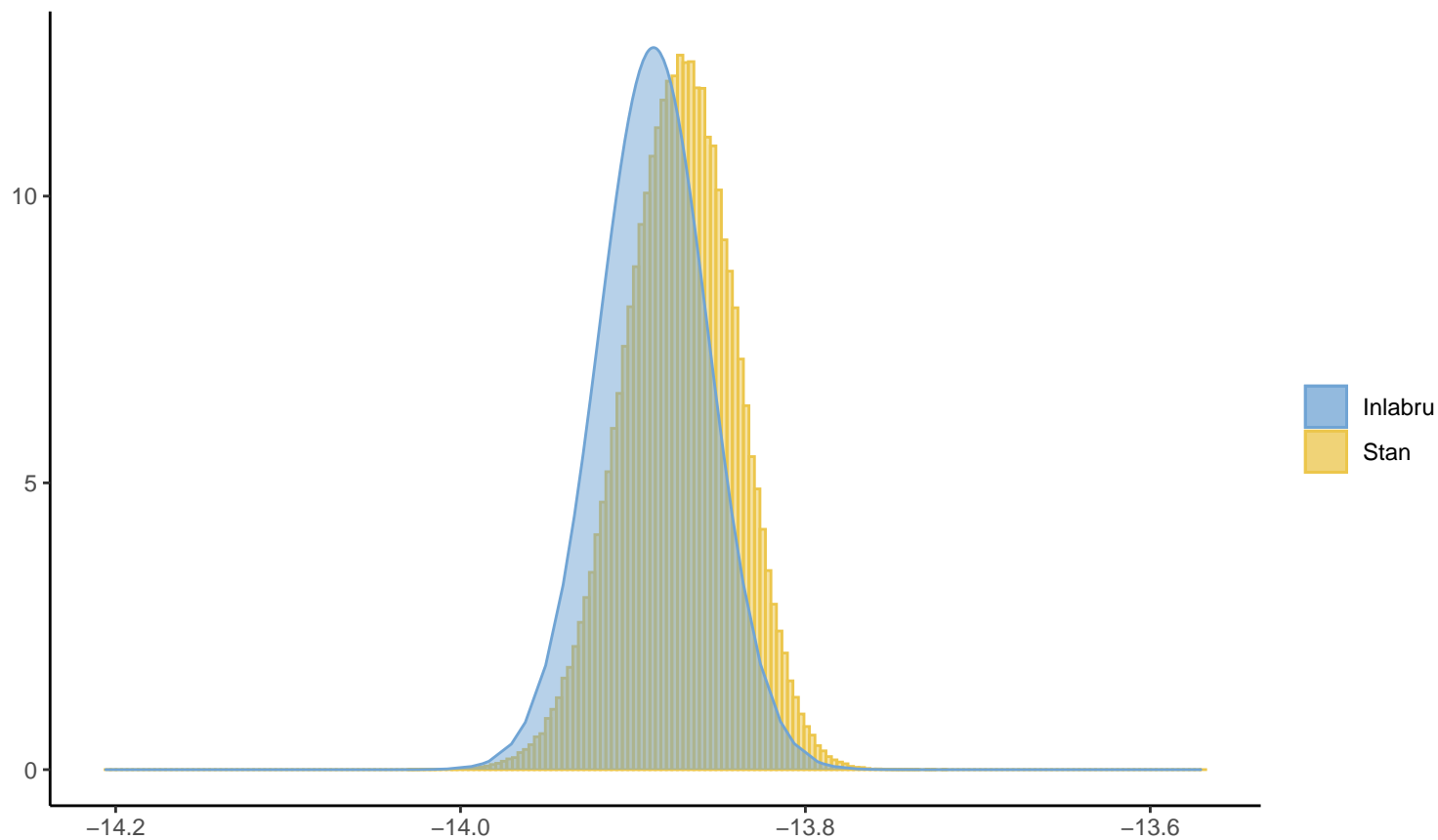
Predictor at xt=36
