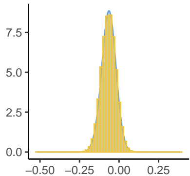
Epsilon[192]
