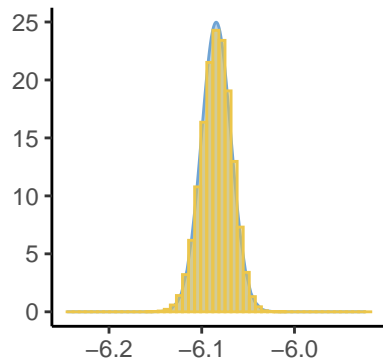
Predictor[96]
