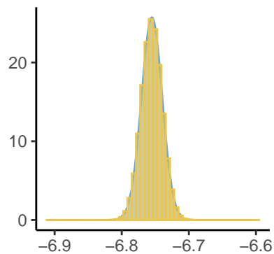
Predictor[32]
