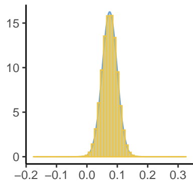
Epsilon[1]
