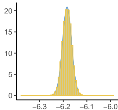
Predictor[64]
