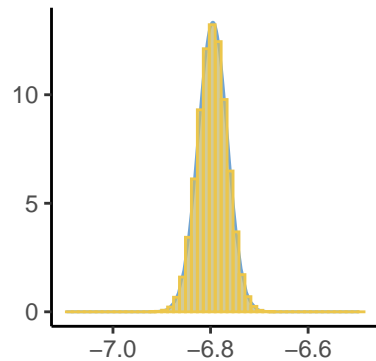
Predictor[162]
