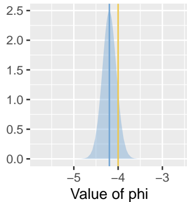
Phi*t + kappa
