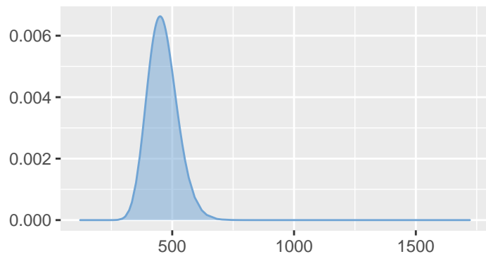
Precision of epsilon
