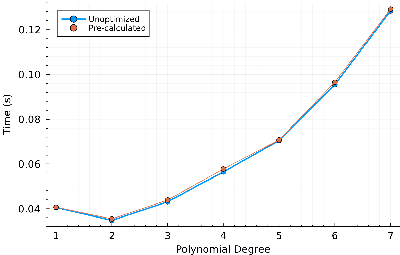
Average runtime per iteration as a function of the Polynomial Degree
