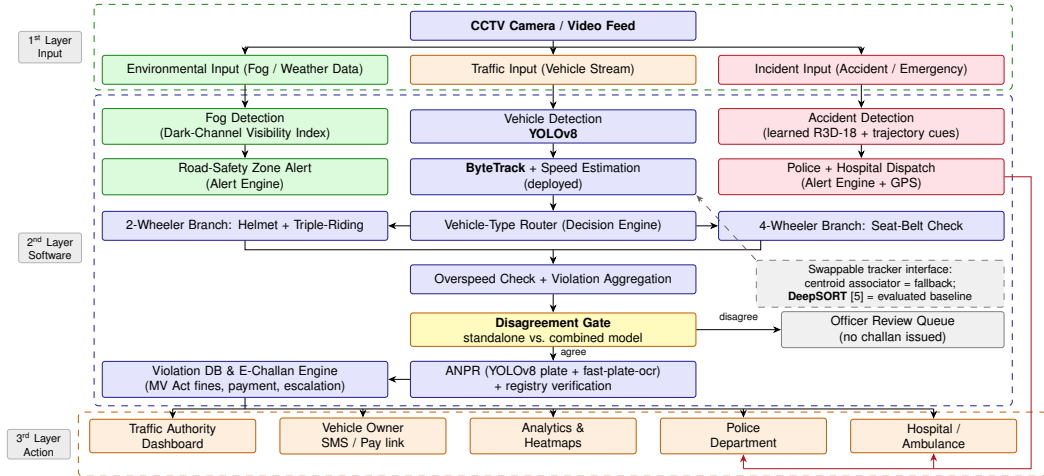
Fig. 1: DriveShieldX system architecture. The deployed configuration tracks with ByteTrack; the centroid associator is the fallback at the same interface and DeepSORT is implemented as an evaluated baseline. The disagreement gate is the single point at which an automatic challan can be suppressed in favour of human review, and only a registry-verified plate leads to an automatic challan.
