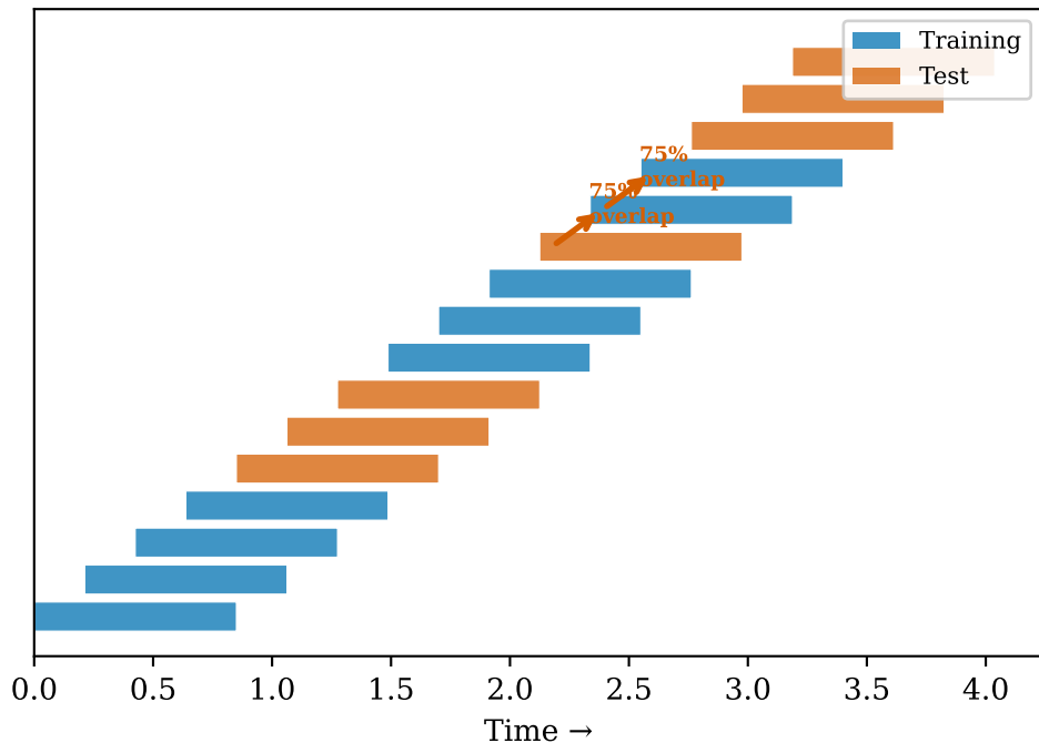
Random Split (Current Standard — Leakage)
