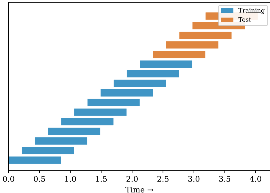
Temporal Split (TSP — No Leakage)
