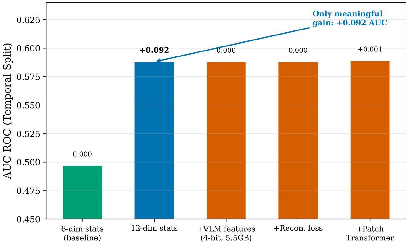
Figure 3 | What Drives Detection Performance?
