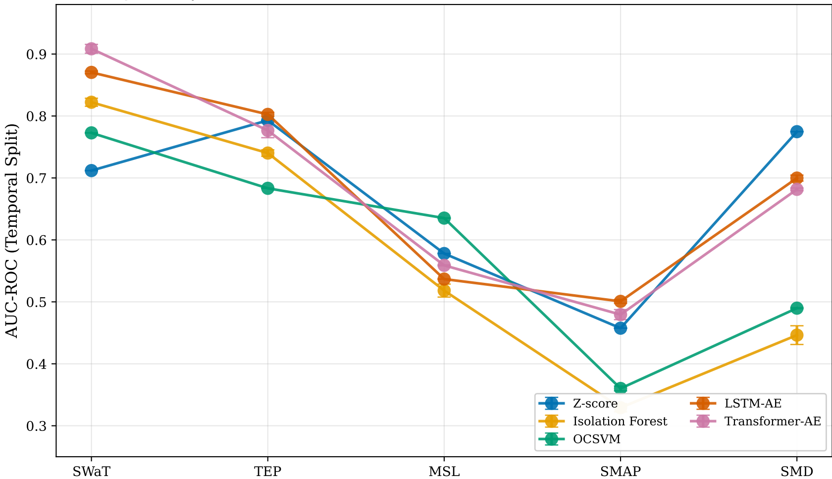
Figure 4 | Honest Evaluation: Detection Performance Under Temporal Split
