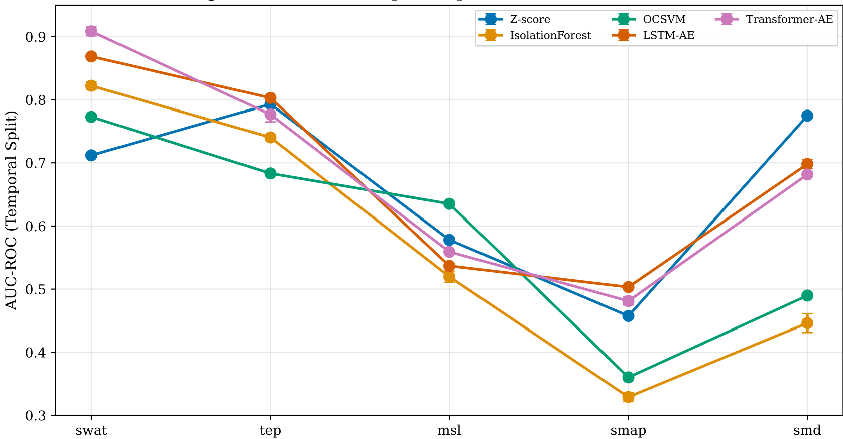
Figure 4: Honest (Temporal-Split) Detection Performance
