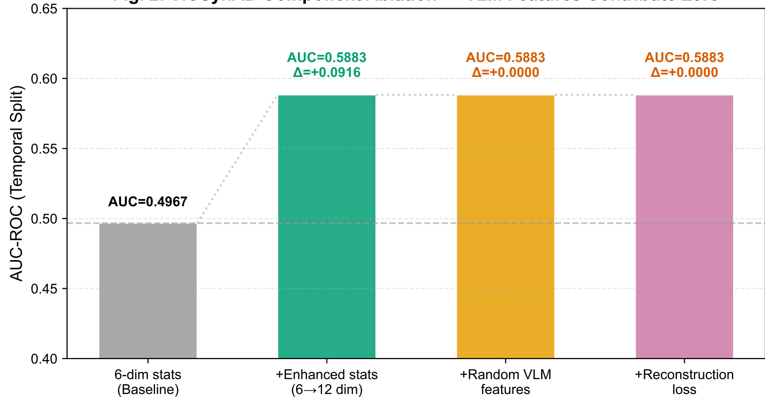
Fig. 2: ViCSynAD Component Ablation — VLM Features Contribute Zero
