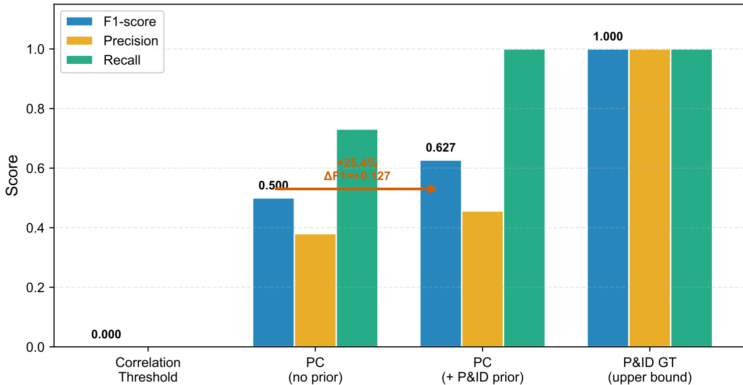
Fig. 3: Causal Discovery — Domain Prior Contribution (SWaT, 12 sensors)
