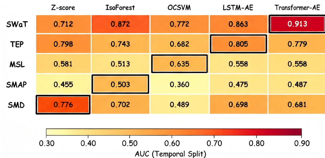
(e) Honest Temporal-Split AUC Matrix (Higher is Better)
